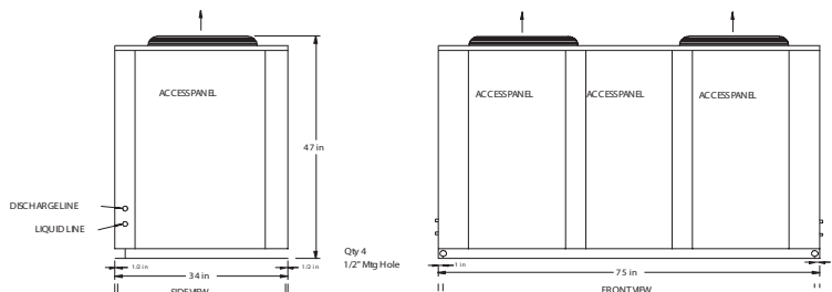
Condenser Model (OC11S)
