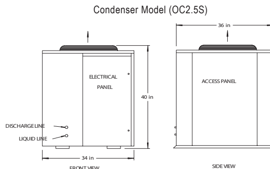
OC Refrigerant Connections: Discharge Line- 1/2", Liquid Line- 3/8"
