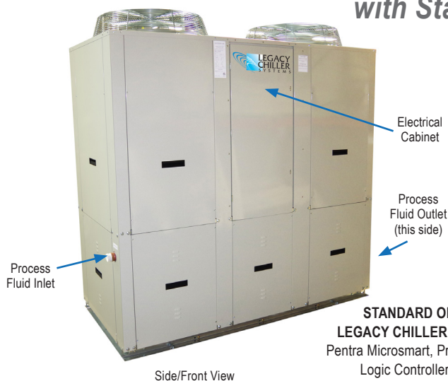
Side/Front View
